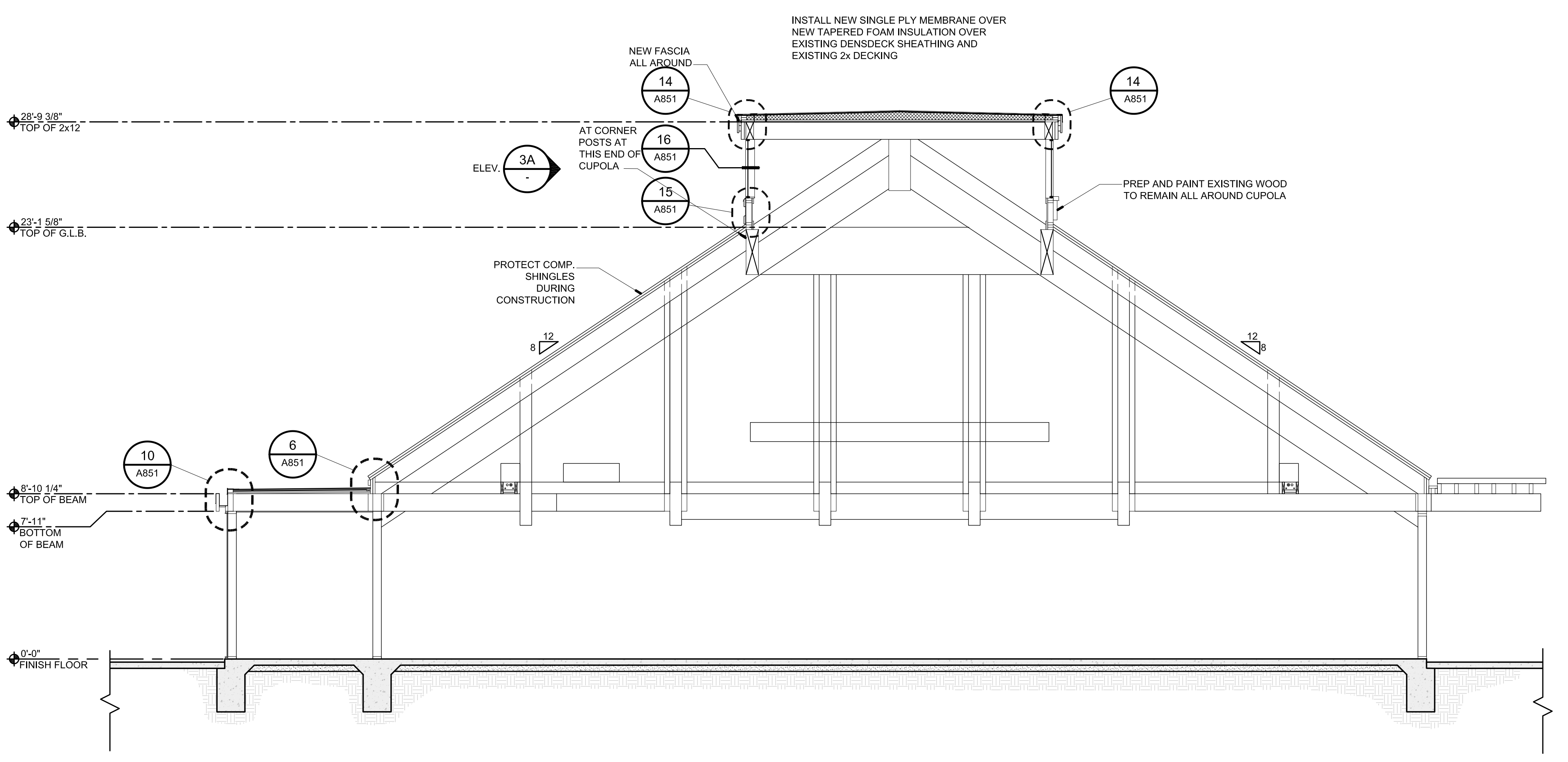
3 TRANSVERSE BUILDING SECTION
